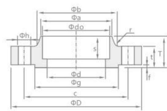
SW of nominal size 10A to 80A
