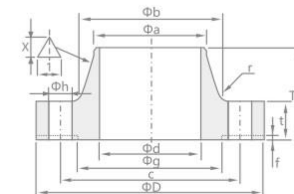
WN of nominal size 15A to 400A
