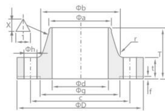
WN of nominal size 10A to 600A
