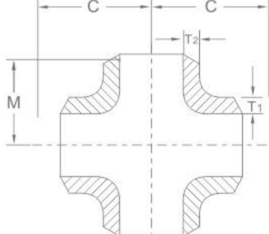
等径四通 Straight Outlet Cross
