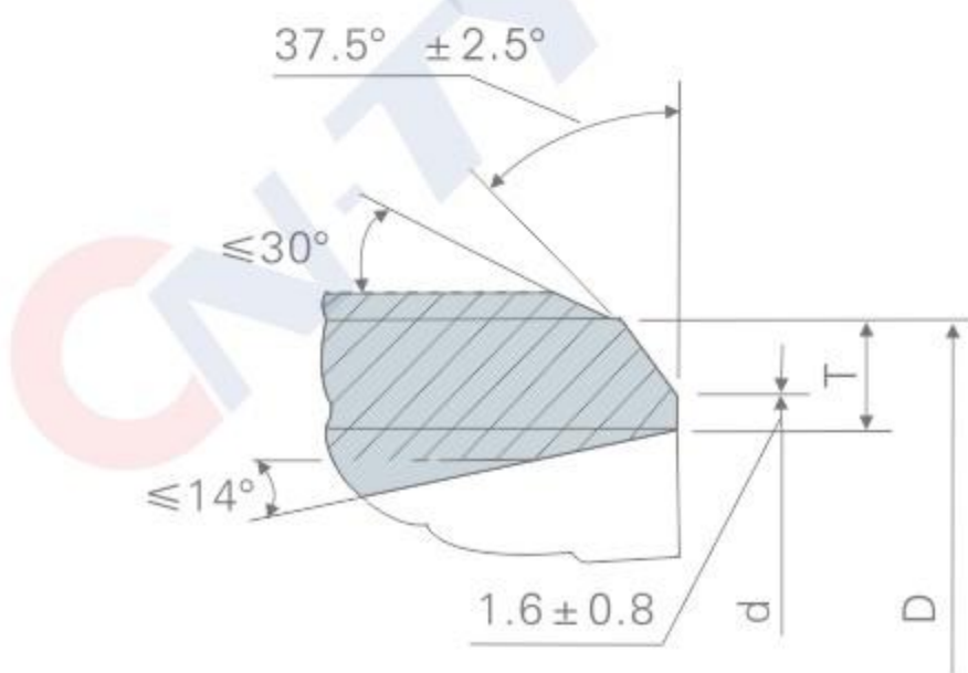
(a) 壁厚 ≤ 22
