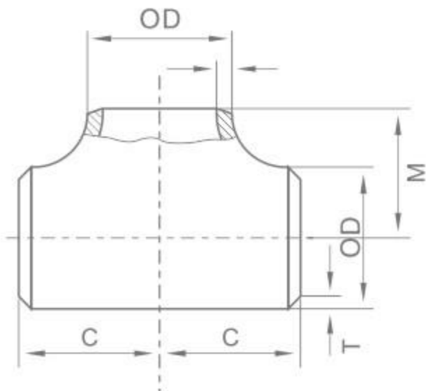
等径三通 Straight Outlet Tee
