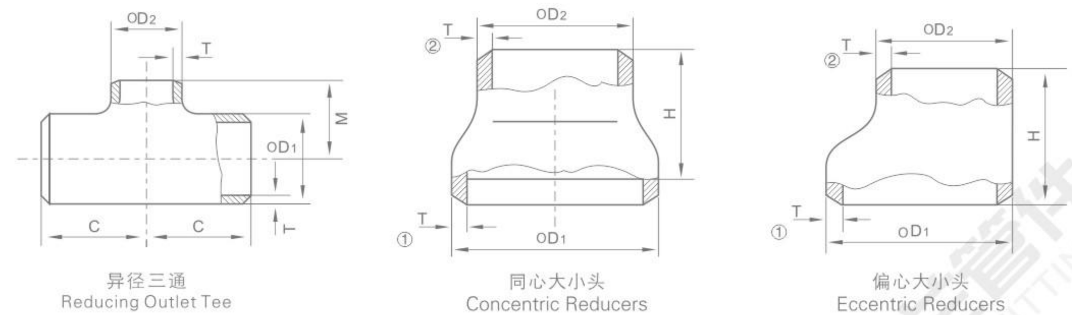
ASME B16.9
