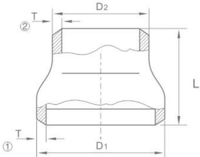
同心大小头 Concentric Reducers
