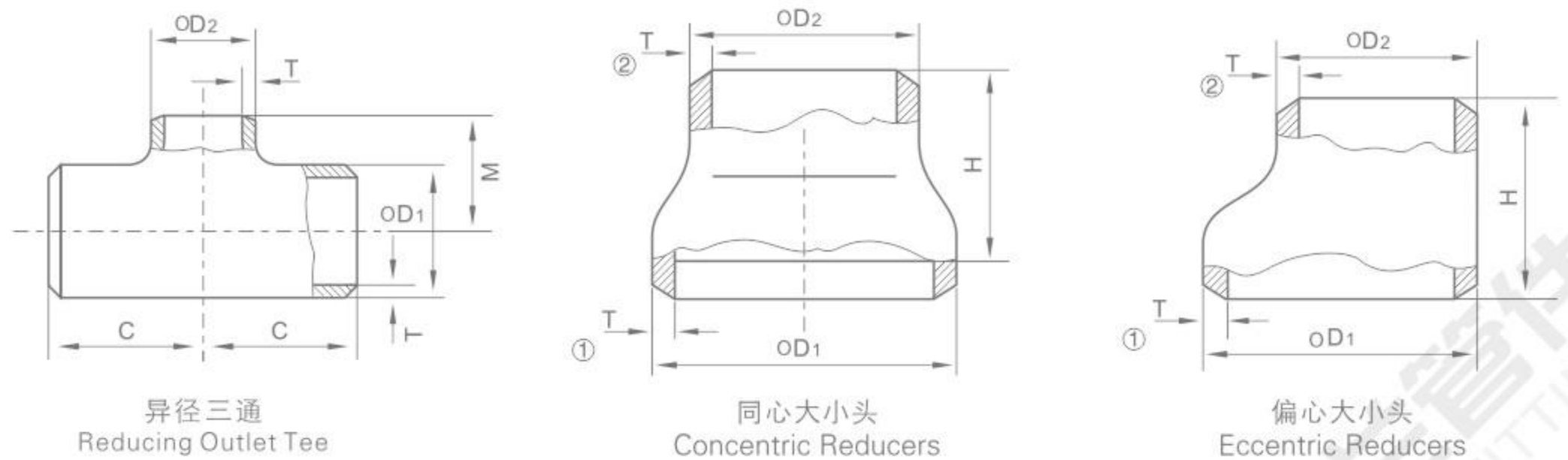
ASME B16.9
