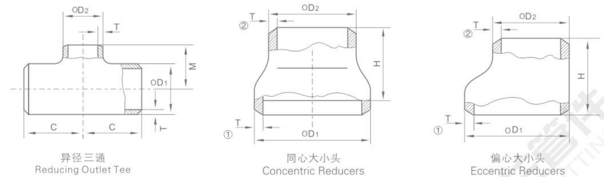
ASME B16.9
