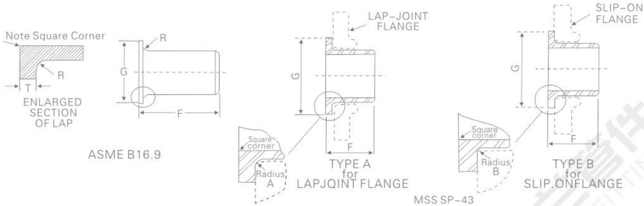
ASME B16.9 MSS SP-43
