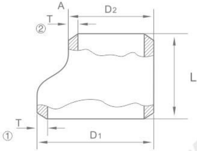
偏心大小头 Eccentric Reducers
