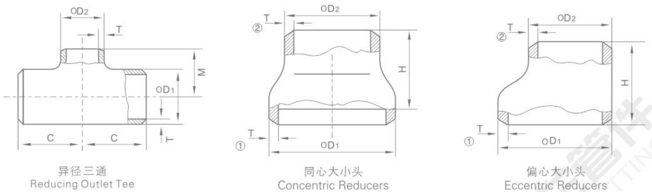
ASME B16.9
